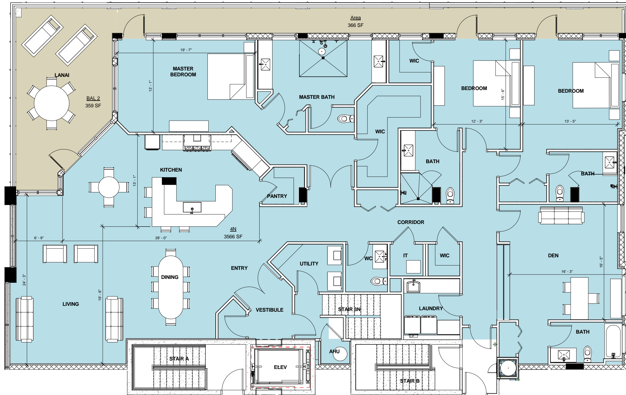
1 LEVEL 4 - UNIT 4N 1/4" = 1'-0"
